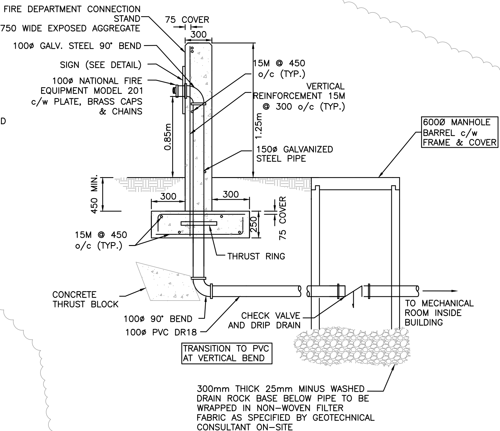
REMOTE SIAMESE FIRE DEPARTMENT CONNECTION DETAIL
