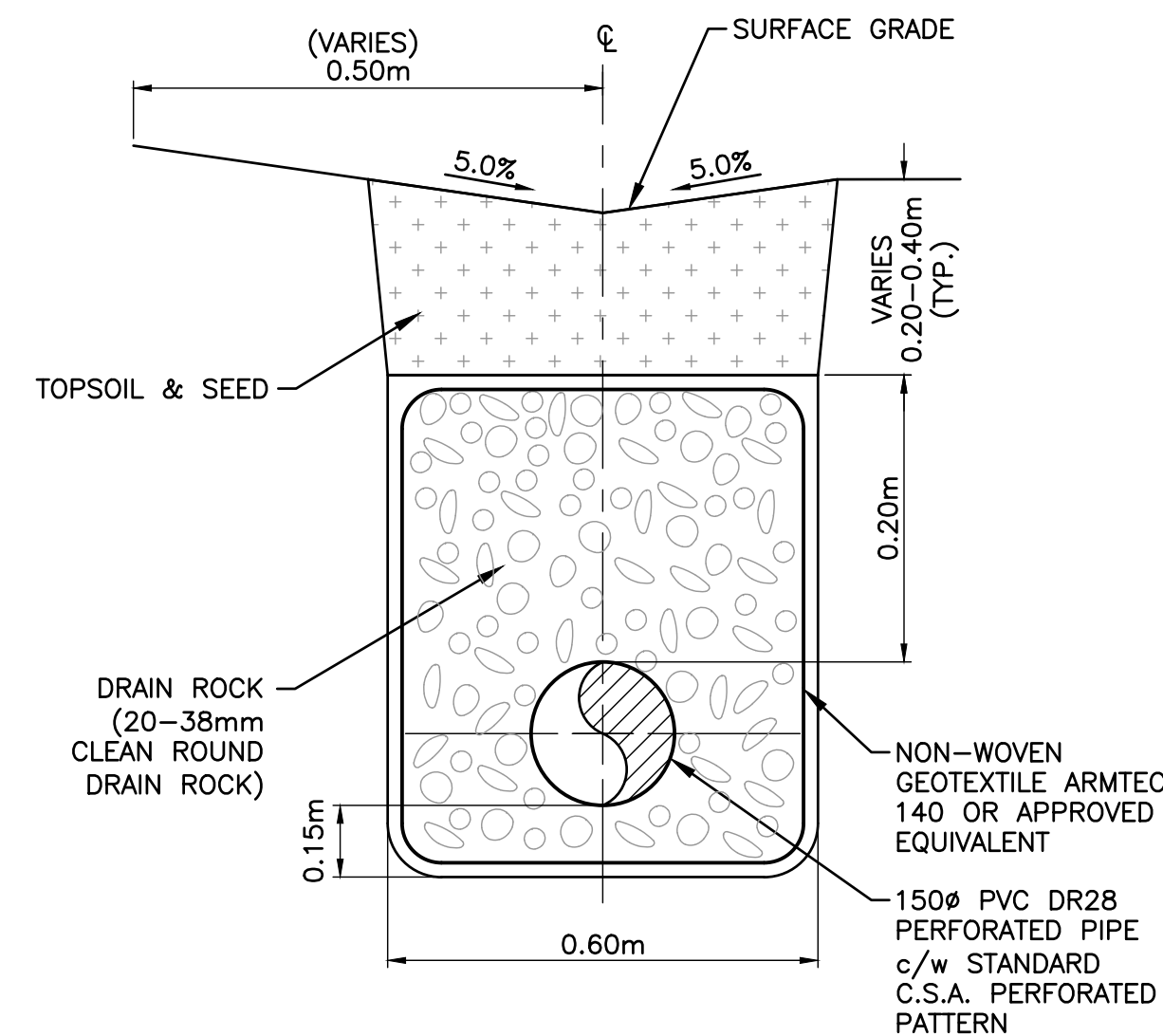
FRENCH DRAIN DETAIL
