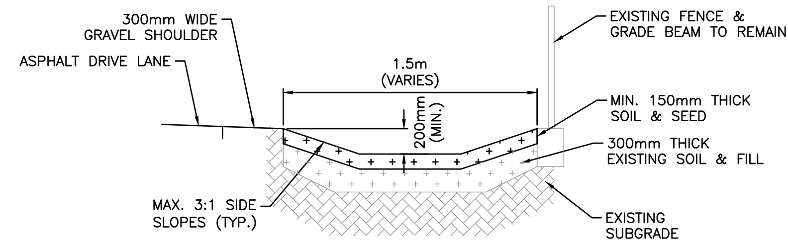
TYPICAL SWALE CROSS SECTION
